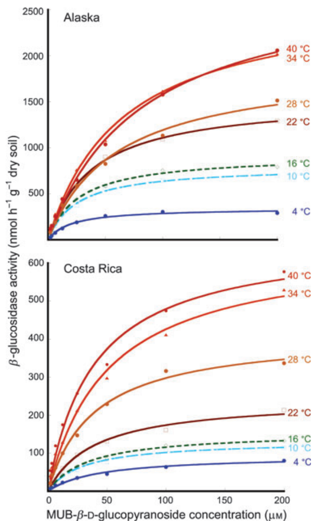
Fig. 1 Michaelis–Menten plots (enzyme activity as a function of substrate concentration) of \beta -glucosidase measured at seven different temperatures in Alaskan and Costa Rican soils. The line observed at each temperature is labeled. Values are means and errors were deliberately not included for clarity. The full name of the substrate is methylumbelliferyl- \beta -D-glucopyranoside.
