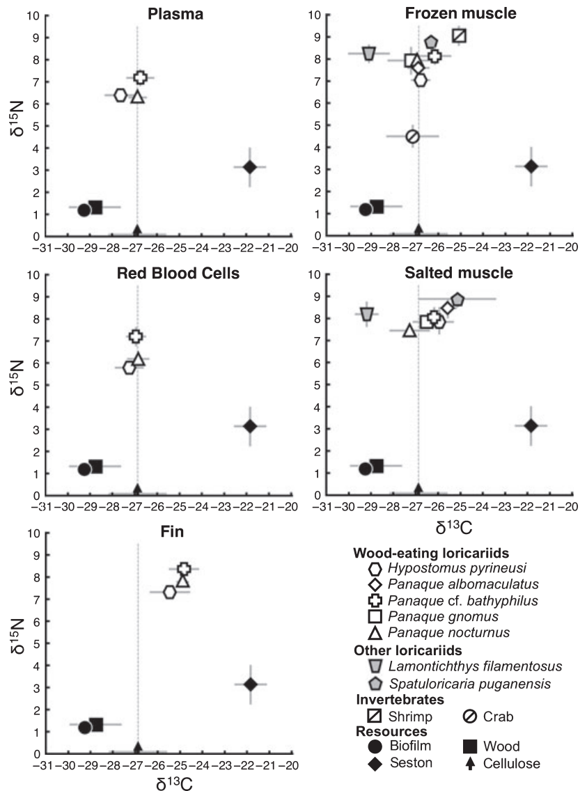
Fig. 2. Distributions in \delta^{13}\text{C} vs. \delta^{15}\text{N} biplot space of various tissues sampled from individuals of seven loriciiid species, shrimps, crabs, biofilm scraped from wood, bulk wood, seston and holocellulose purified from bulk wood. Vertical dashed line marks the mean position along the \delta^{13}\text{C} axis of purified holocellulose. Values represent mean \pm standard deviation. Numbers of sampled individuals given in Table 1.
